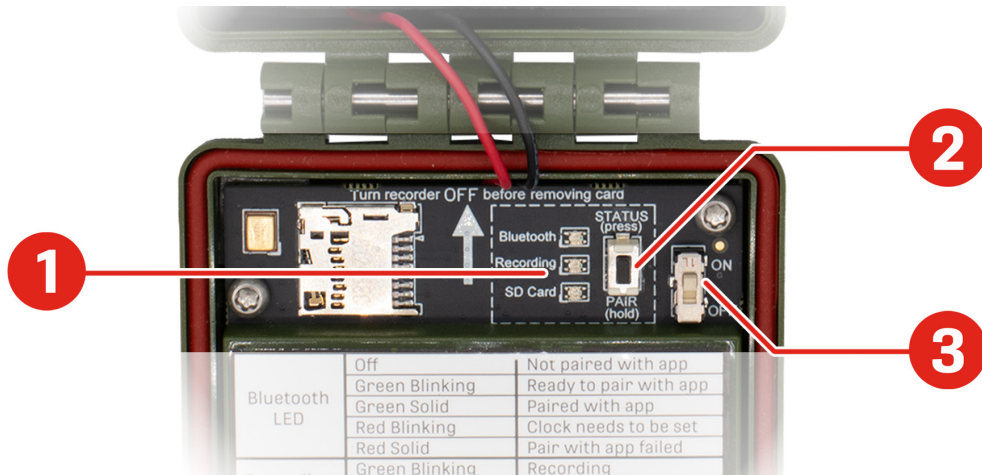
Figure 6. Control Panel
